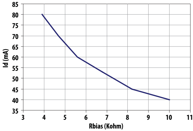
Figure 28. Id vs Rbias
